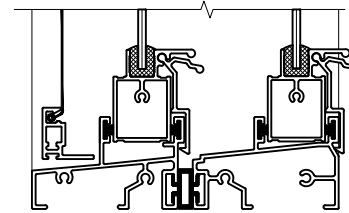
260 DOUBLE HUNG
