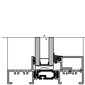
230 FIXED WINDOW
