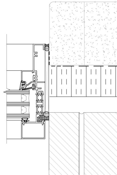
Jamb detail - triple glazed
