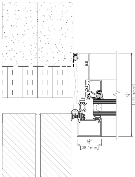
Jamb detail - double glazed
